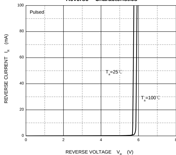
Reverse Characteristics
