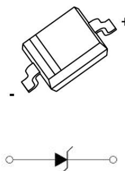
SOD-323
