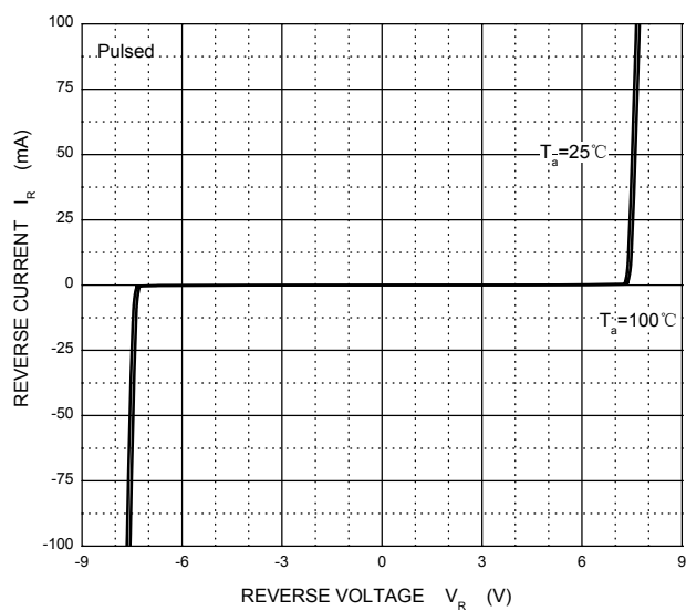
Reverse Characteristics
