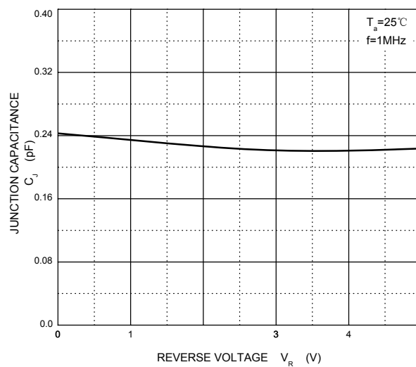
Capacitance Characteristics
