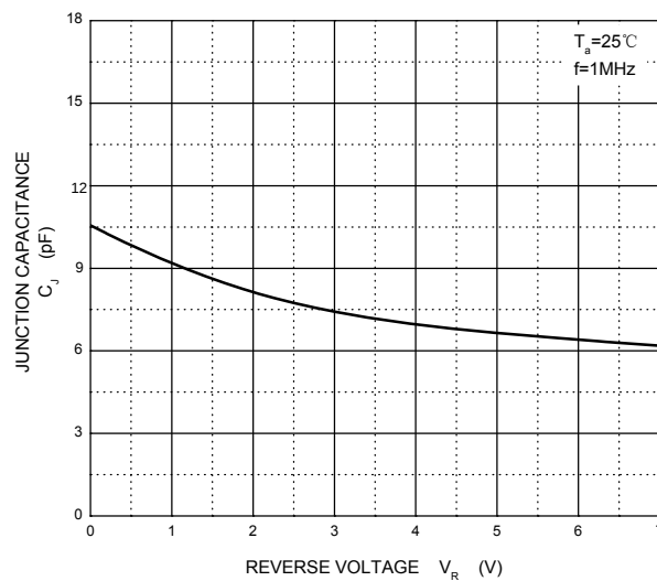
Capacitance Characteristics
