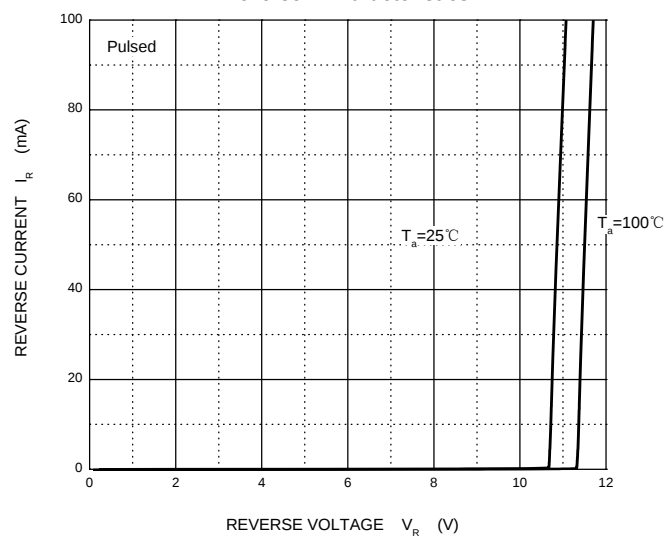
Reverse Characteristics
