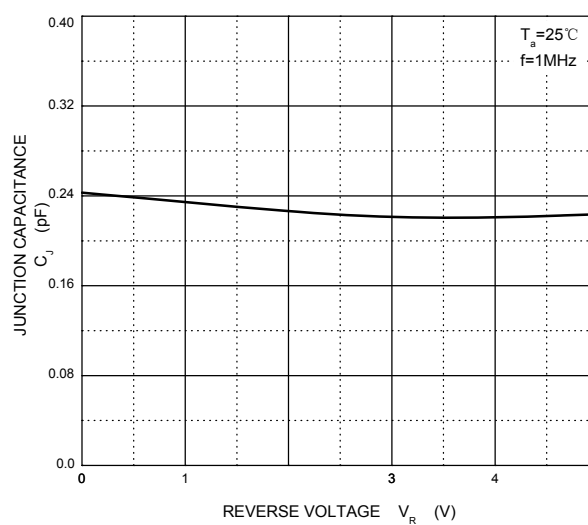
Capacitance Characteristics
