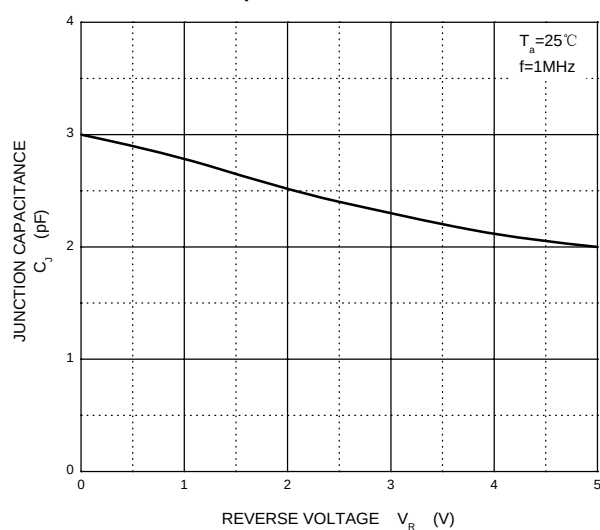
Capacitance Characteristics
