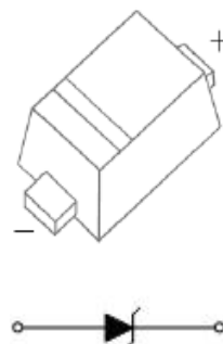
SOD-523
