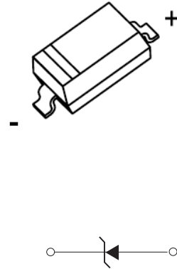
SOD-123
