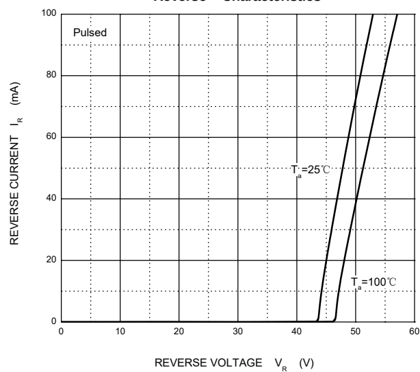
Reverse Characteristics
