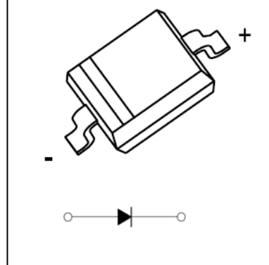
SOD-323
