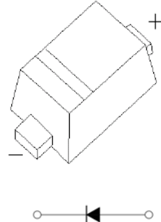
SOD-523
