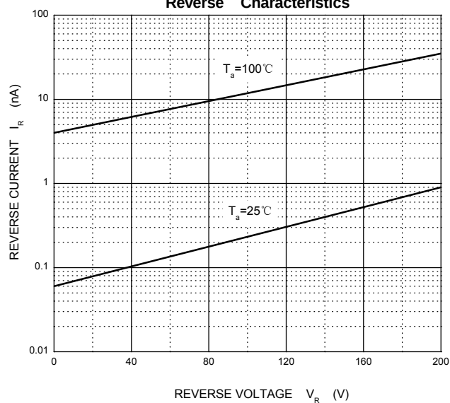
Reverse Characteristics
