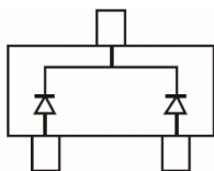
BAS40-05T MARKING: 45
