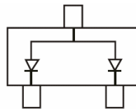
BAS40-06T MARKING: 46
