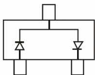
BAS40-04T MARKING: 44
