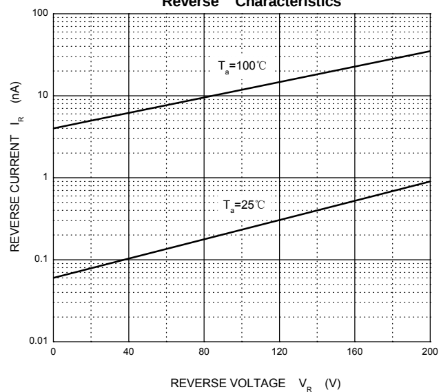
Reverse Characteristics
