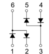
BAT54SDW
