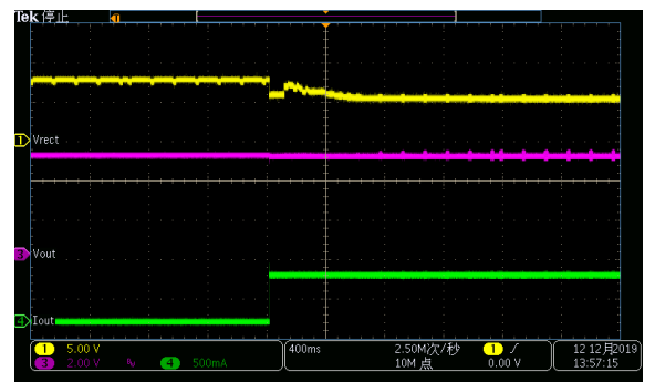
Figure4. Transient Resp: V_{out}=5V ; I_{out}=0 to 0.6A
